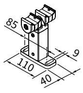
11 double track bracket with adjustable head 140 mm 12 central bracket for 2 single units next to each other
