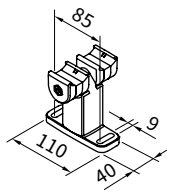
06 double track bracket with adjustable head 100 mm 07 central bracket for 2 single units next to each other
