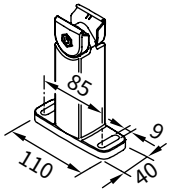
09 track bracket, with adjustable head 140 mm
