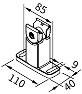
03 track bracket, with adjustable head 04 100 mm
